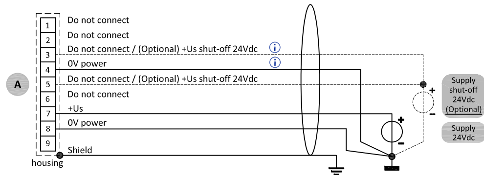
9 pin D-Sub connector cable part female
