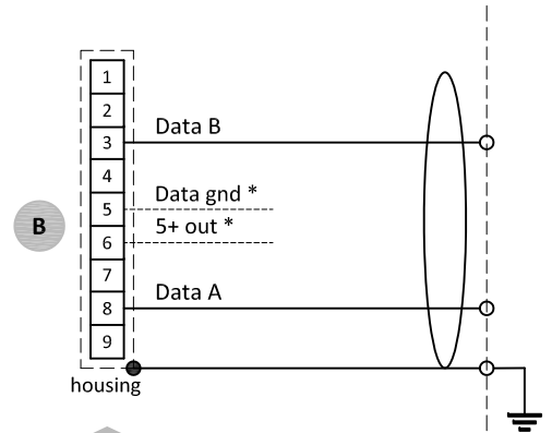
9 pin D-Sub connector cable part male
