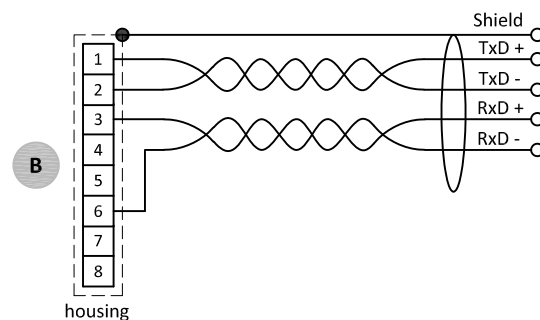
RJ45 modular jack cable part male
